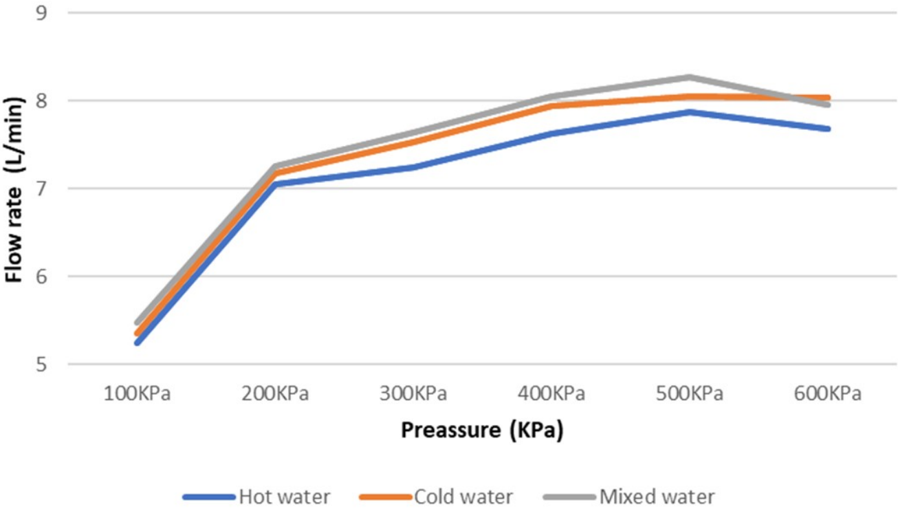
Flow Rate (L/min): SE-951R-BN
